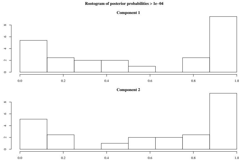
Figure 4: plot(m3)
