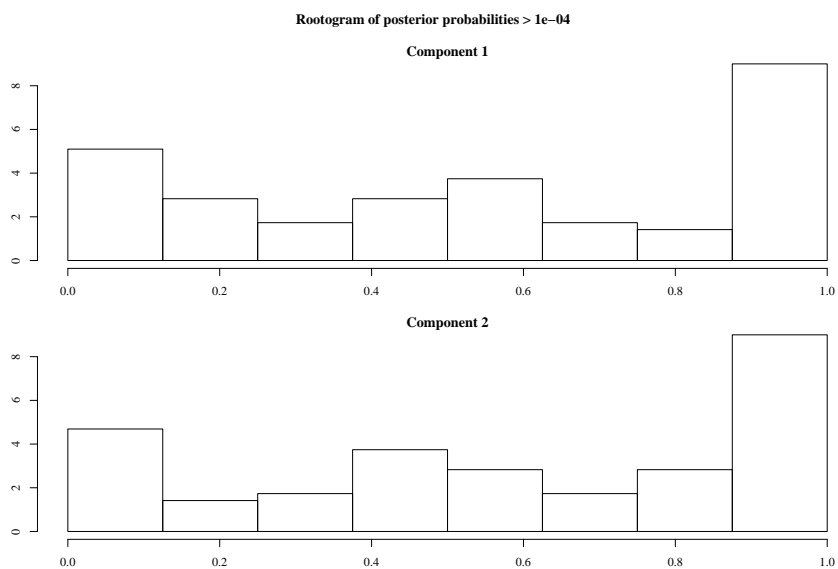
Figure 2: plot(m1)
