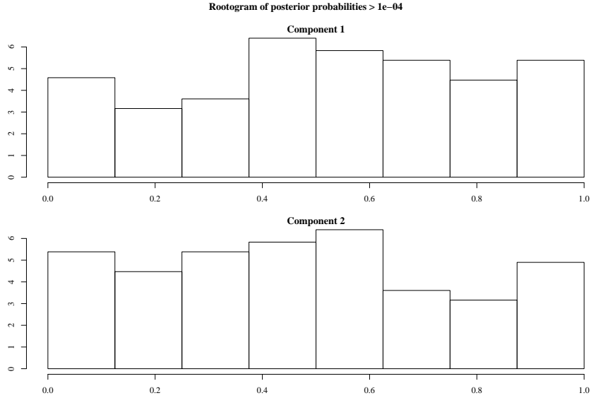
Figure 3: plot(m2)
