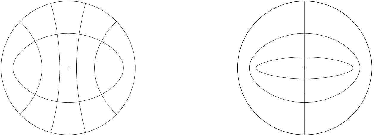
FIGURE 4: NODAL LINES OF u_{00} (LEFT HAND SIDE) AND u_{10} (RIGHT HAND SIDE) IN STEREOGRAPHIC PROJECTION OF THE NORTHERN HEMISPHERE (THE CROSS MARKS THE POLE).
