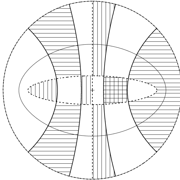
FIGURE 5: p_{00} (THICK LINE), p_{10} (DASHED LINE) (INCLUDES THE EQUATOR) AND THE COMMON CONIC q_1 OF THE PENCIL (THIN LINE) IN STEREOGRAPHIC PROJECTION OF THE NORTHERN HEMISPHERE.
