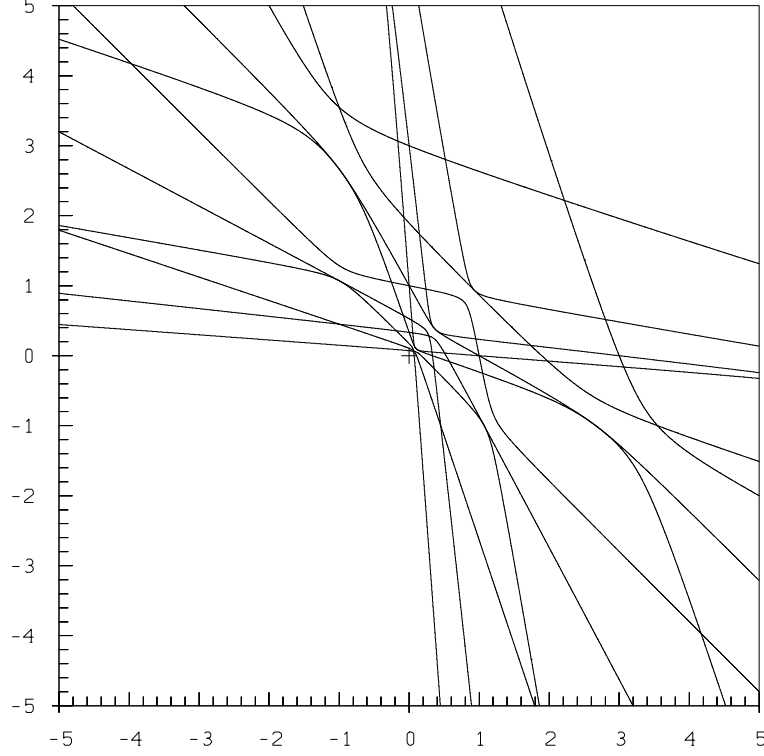
FIGURE 3: THE CURVE \xi_{00} \cdot \xi_{10} \cdot \xi_{01} \cdot \xi_{11} PLOTTED FOR \gamma = -1 , -5 \leq \alpha, \beta \leq 5 .
